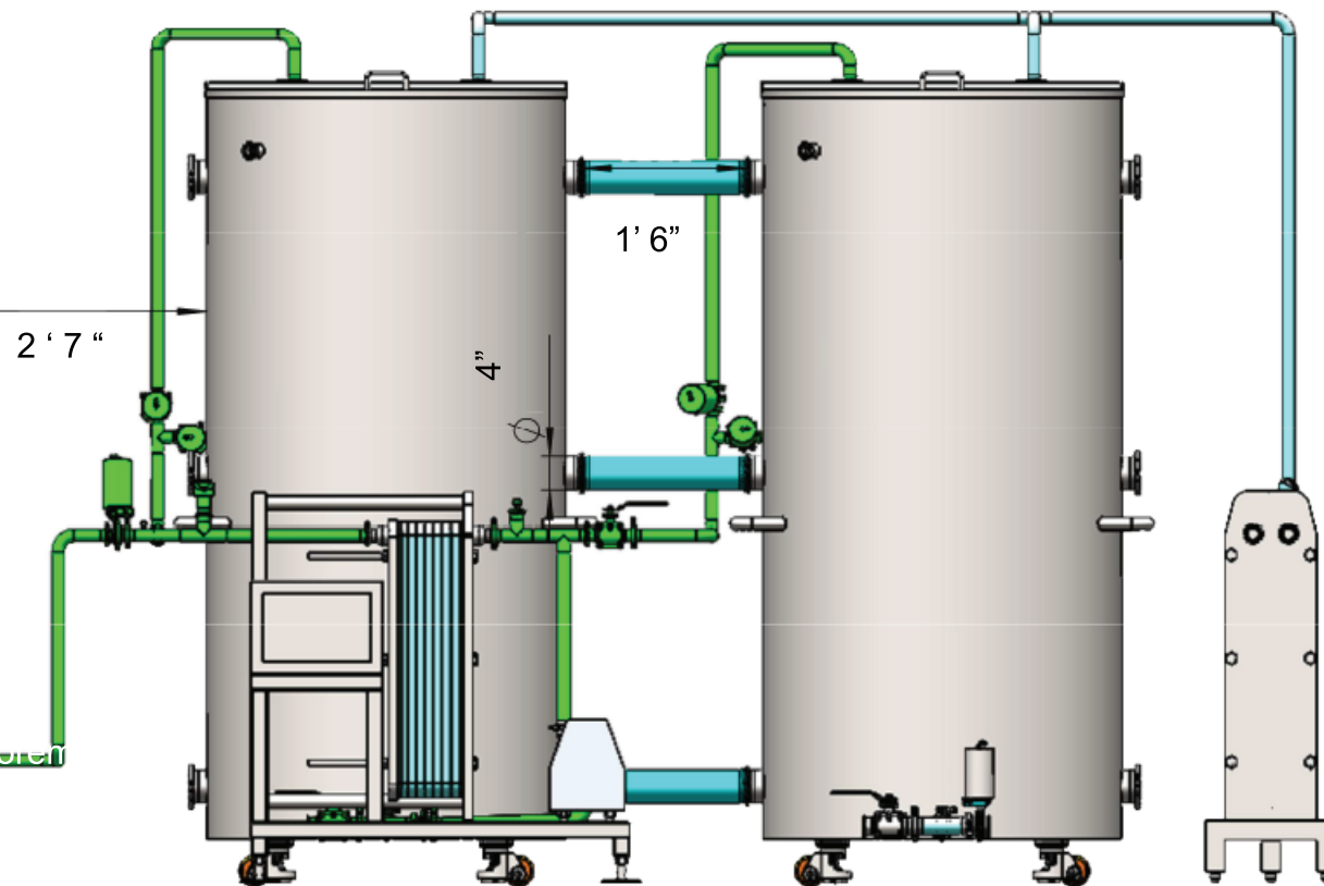
400 Gallon Iced Water Tank #1
